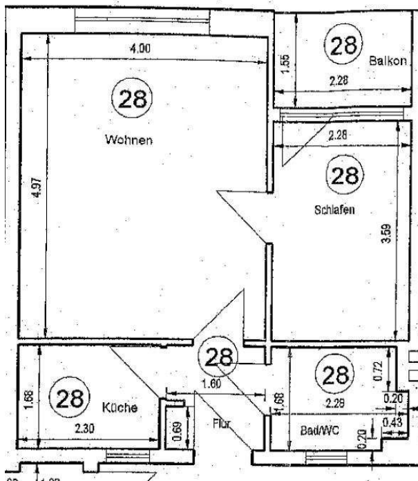
Grundriss WE28
