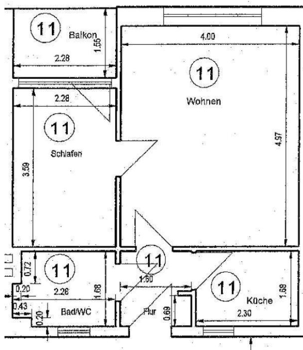
Grundriss WE11
