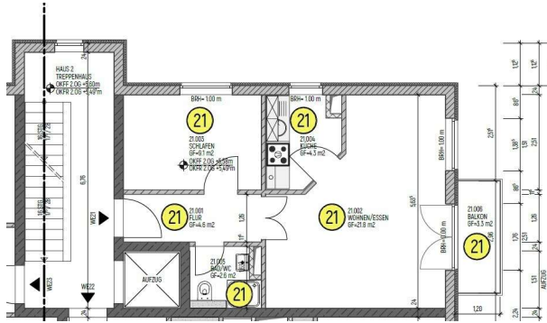
Grundriss WE 21
