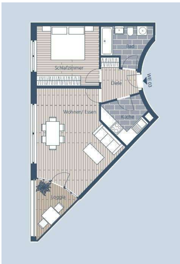
Grundriss WE 3
